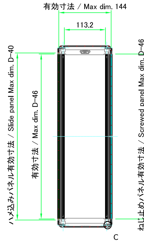
B-B (1:6)
